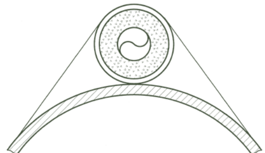
Typical DLS-IT Cross Section (Tracer attached to pipe with FT-1H tape)
